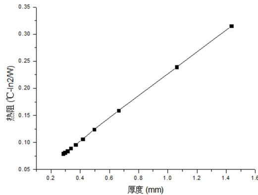
GS-800 Thickness vs Thermal Resistance
