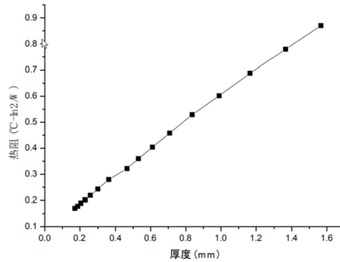
GS-300 Thickness vs Thermal Resistance
