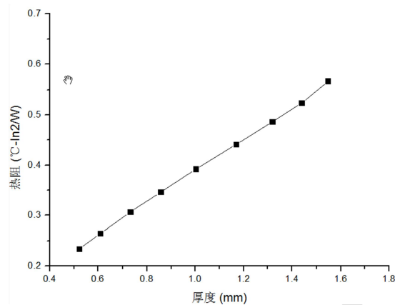
GS-500 Thickness vs Thermal Resistance
